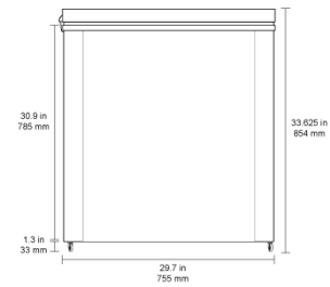
SIDE VIEW (MXSH19.4S & MXSH23.6S)
