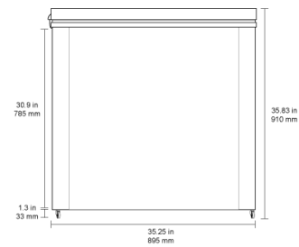
SIDE VIEW (MXSH30.0S)
